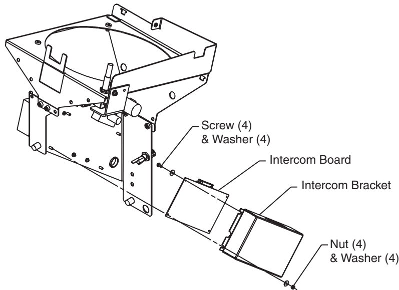
Figure 1 Intercom Assembly
